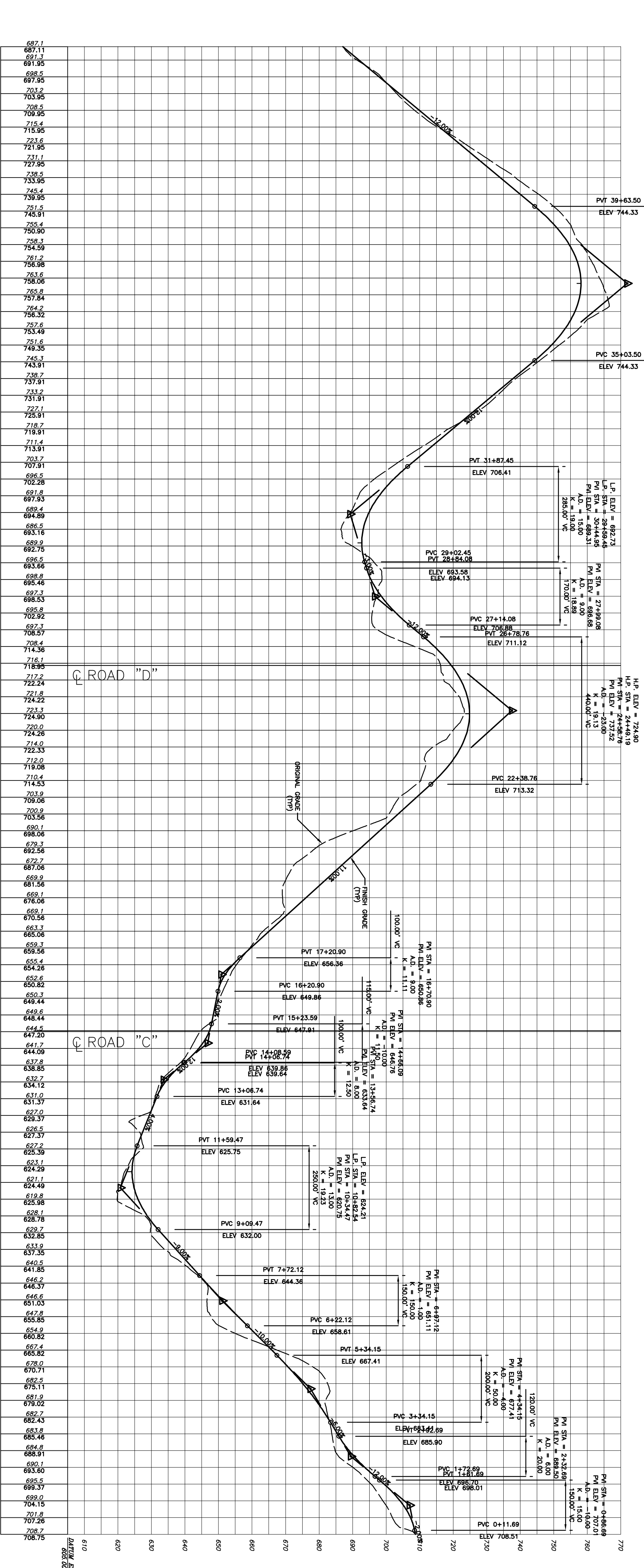
ROAD "C" SCALE: HORIZ 1"=200' VERT 1"=20'
